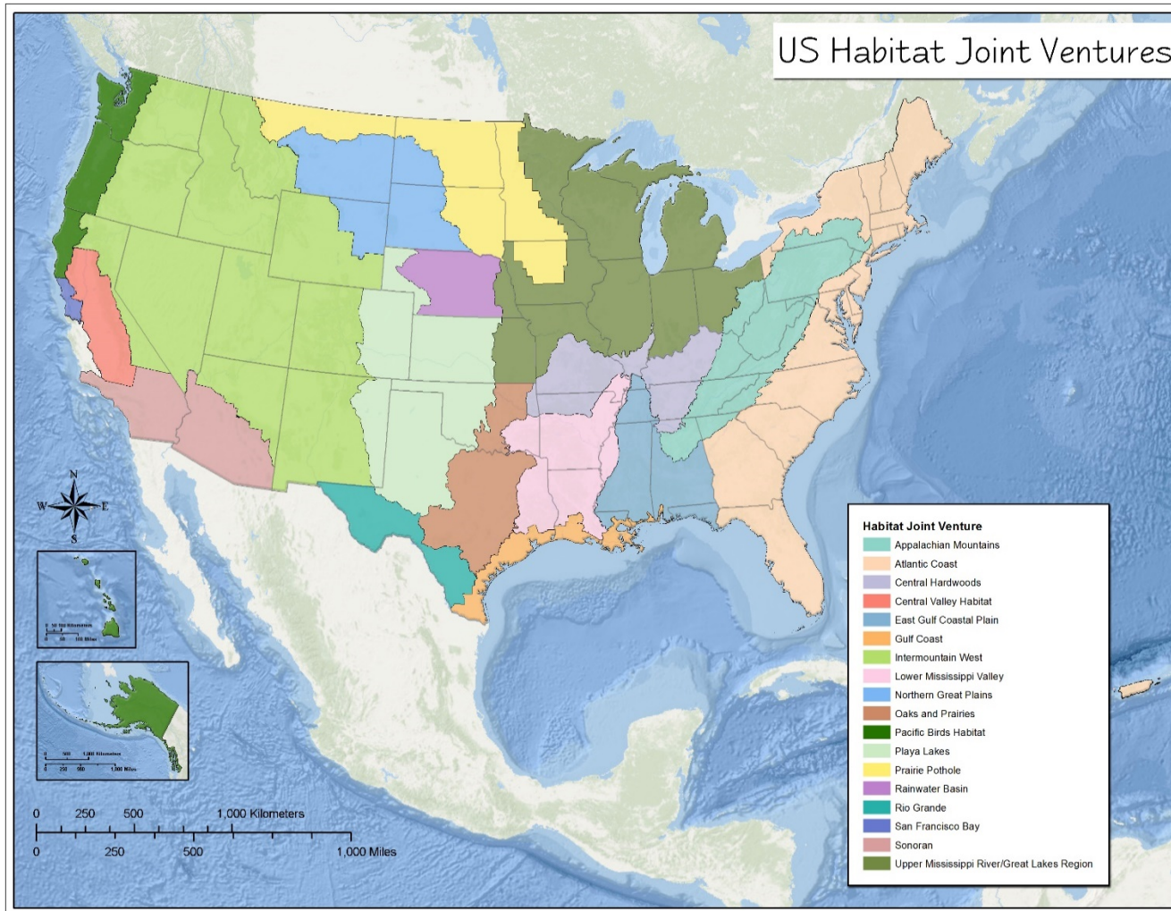
Figure 6: U.S. Migratory Bird Habitat Joint Venture Map
