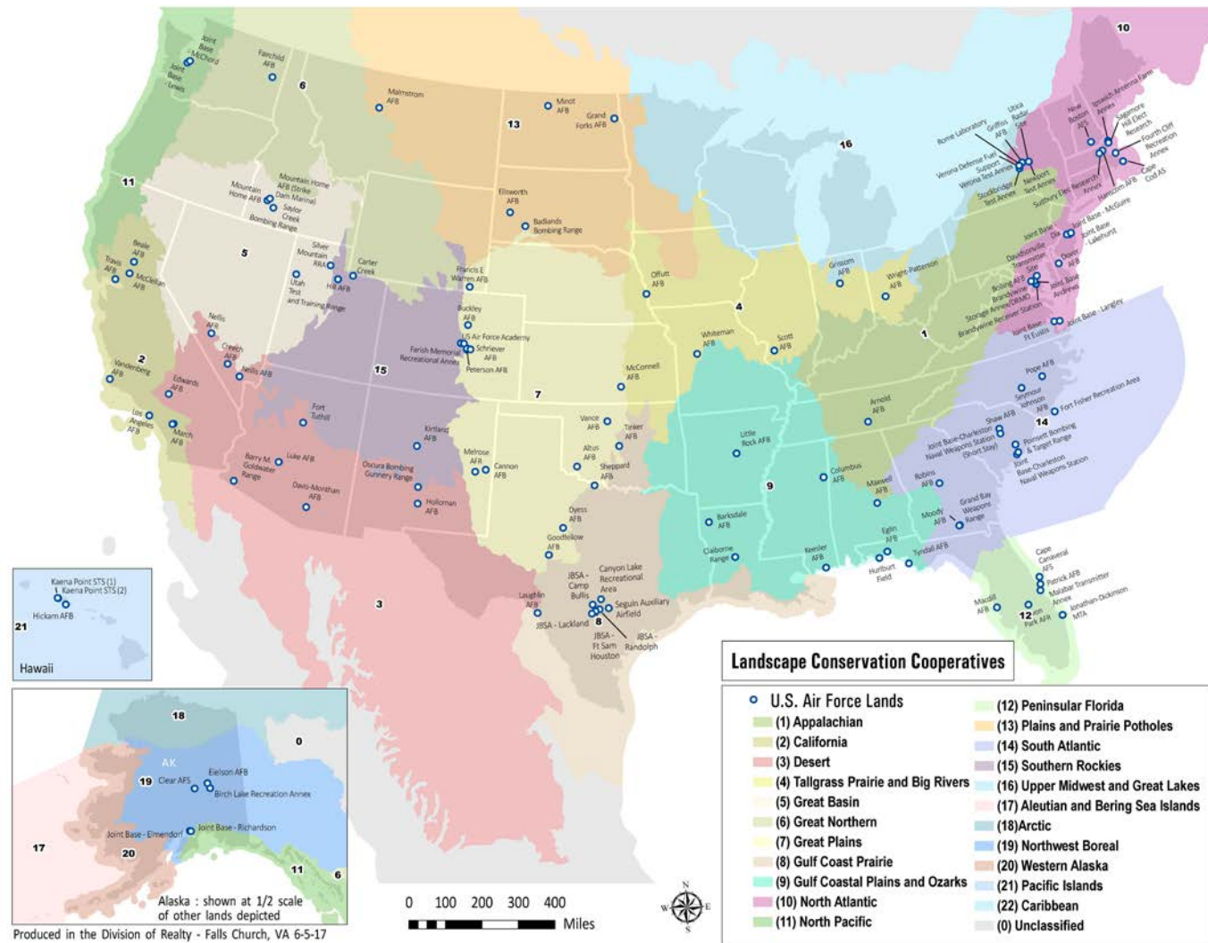
Figure 7: Landscape Conservation Cooperative Network Map
